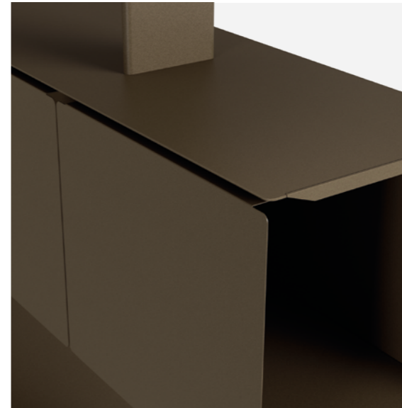
03. Panel The panels are housed between shelves and can be placed interchangeably in front of and behind the shelf. The shelves have discrete cavities that act as rails and allow these sliding panels to be anchored.
